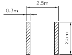
SILO BEARING ARRANGEMENT
